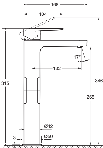
FERLA TALL BASIN MIXER DIMENSIONS
