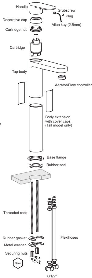
EXPANDED VIEW SHOWING COMPONENTS
