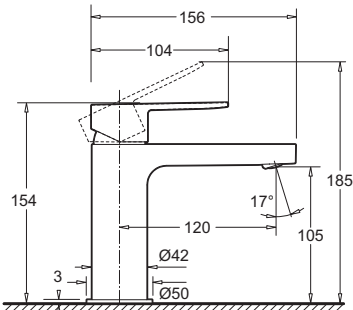
FERLA TALL BASIN MIXER DIMENSIONS
