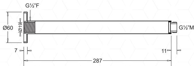
VENEZIA CEILING SHOWER ARM 300mm JTV07
