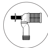
SUPPLIED WITH X011H ADJUSTABLE CONNECTOR FOR S TRAP INSTALLATIONS P TRAP HEIGHT 180mm
